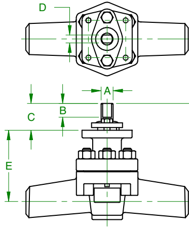
CLASS 600 BUTTWELD STANDARD PORT - SIZES 1/2" THRU 2"
