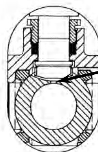
EXAMPLE OF A SLOT VENTED BALL
