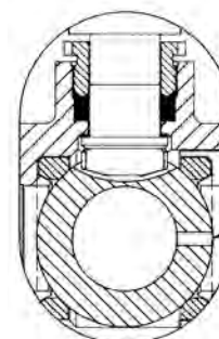
EXAMPLE OF A SIDE VENTED BALL
